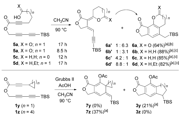
Scheme 3. Double annulation reactions: [a] Yields are those of isolated products. [b] Yield of 6a + 6a' . [c] Yield after complete conversion.
