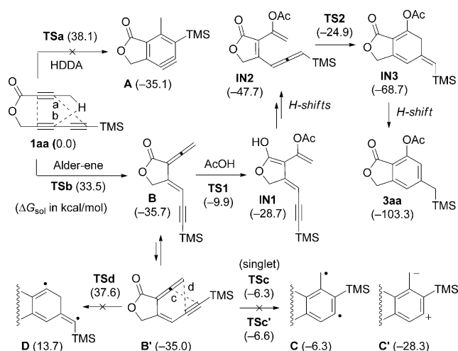
Scheme 2. DFT-based mechanistic rationale. [7]
